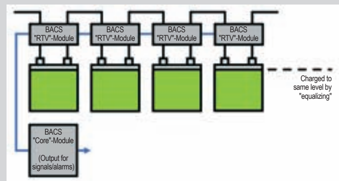
Fig. 3: All batteries attain the same charging level at the end of the charging process, avoiding overcharging or deep discharging of individual batteries and optimising overall capacity.
