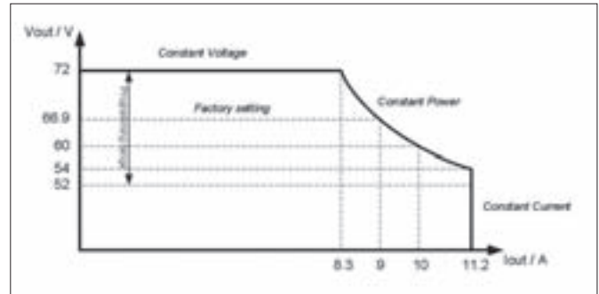
Top picture: Output characteristics 600W, 60V
