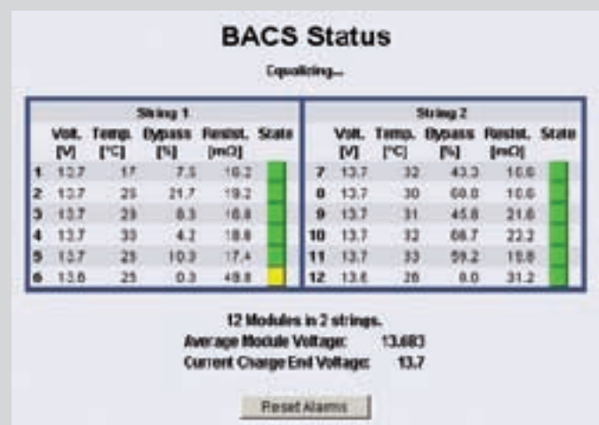
Fig. 4: Remote monitoring of battery systems via BACS and monitoring software increases the system's stability
