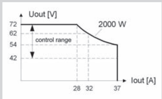
Output characteristic:
